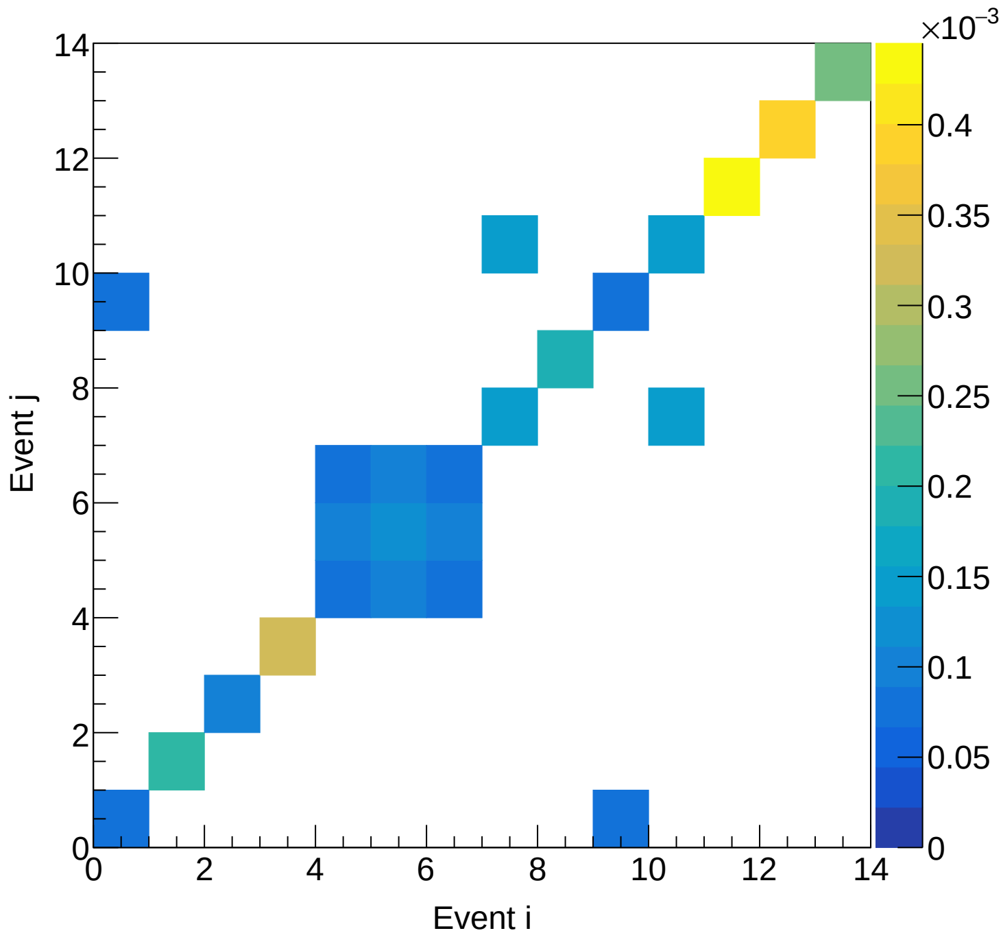
LD2 (total) Covariance | M: [6.0, 6.3) xF: [-0.05, 0.00)
