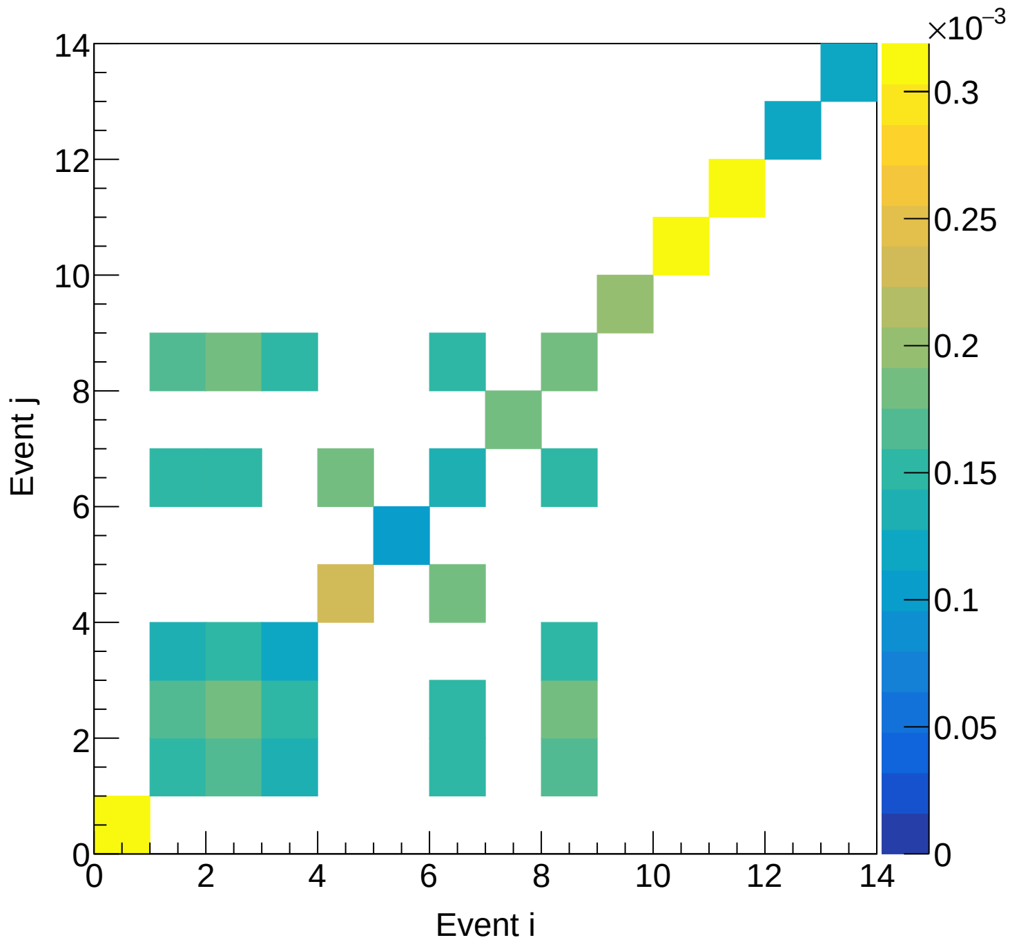
LD2 (total) Covariance | M: [6.3, 6.6) xF: [-0.05, 0.00)
