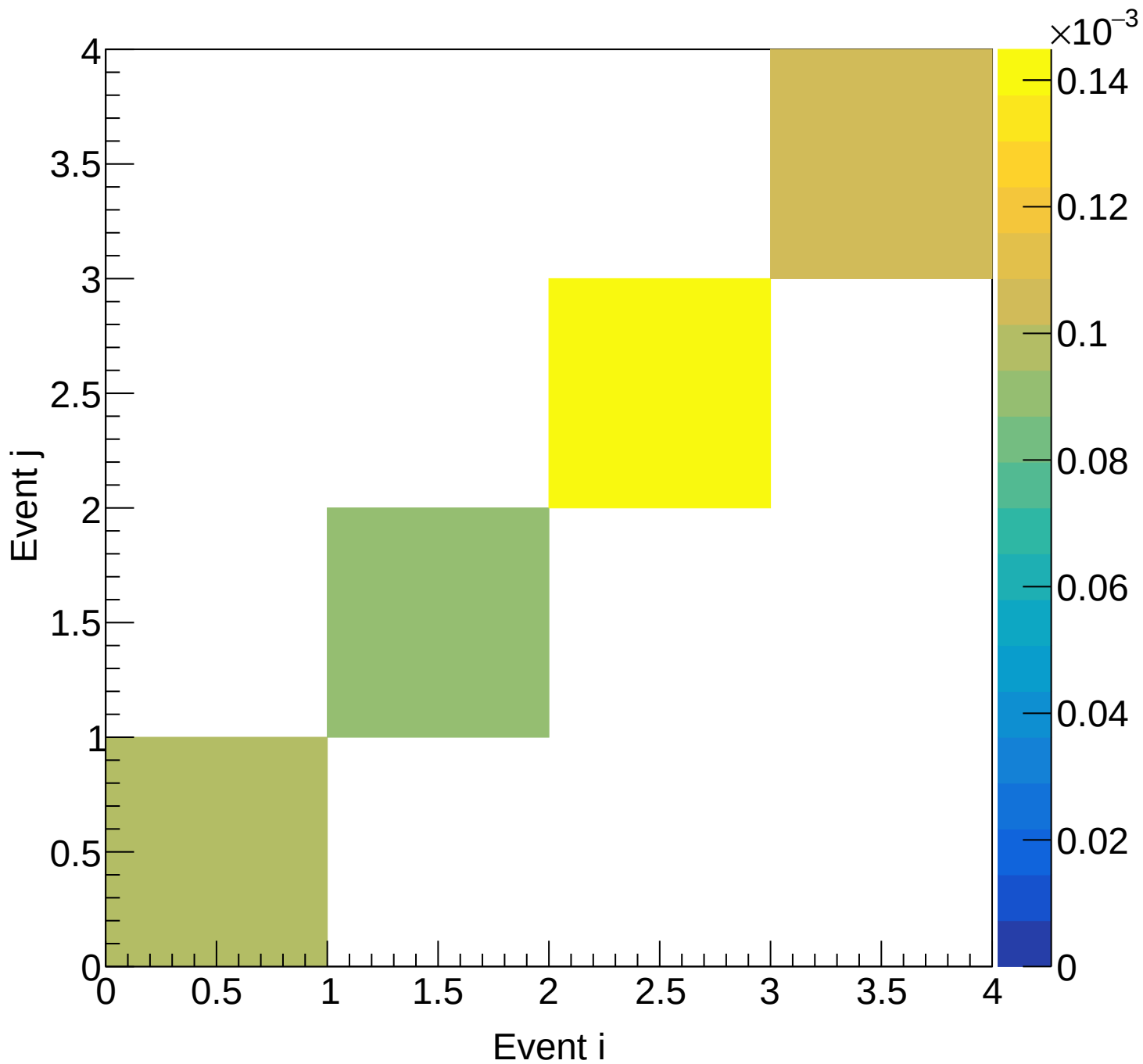
LD2 (total) Covariance | M: [6.6, 6.9] xF: [-0.05, 0.00]
