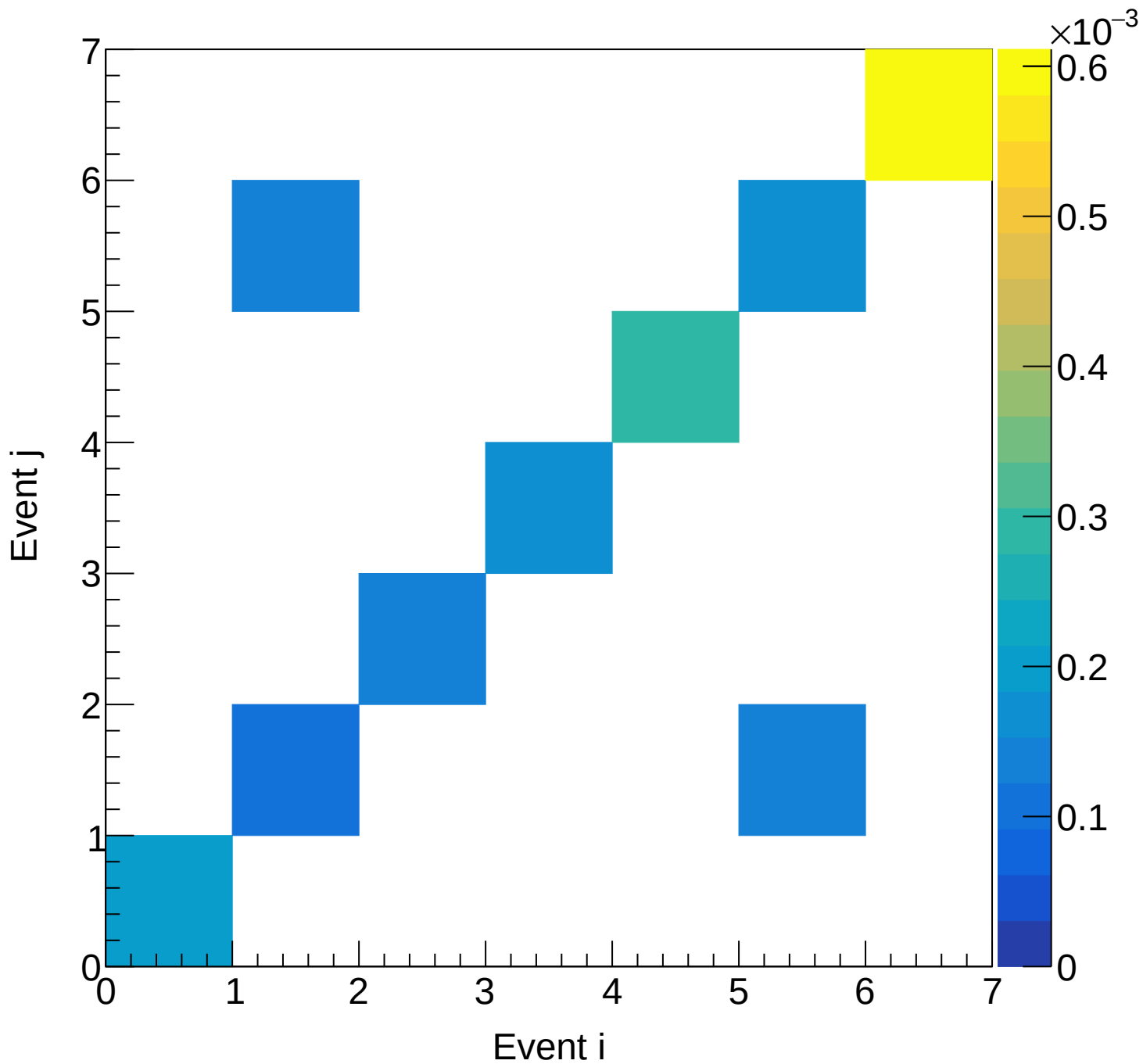
LD2 (total) Covariance | M: [7.5, 8.8) xF: [0.45, 0.50)
