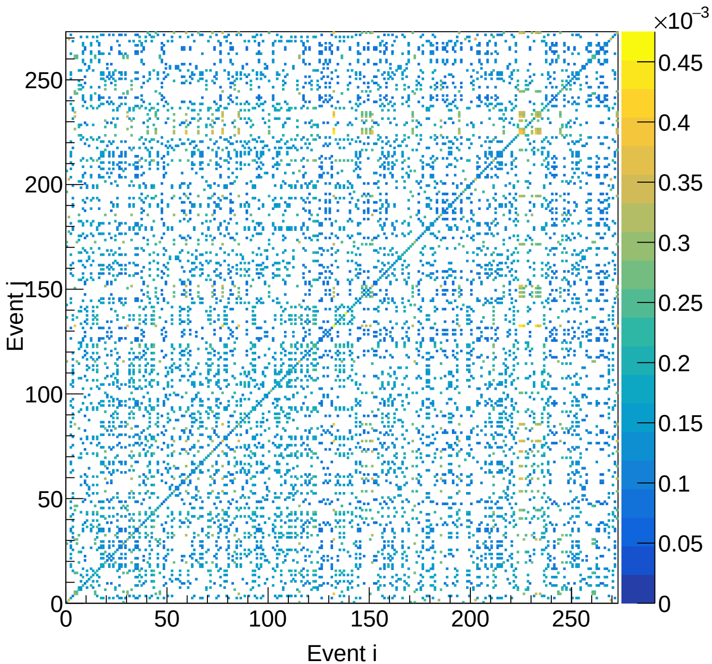
LD2 (total) Covariance | M: [5.1, 5.4) xF: [0.45, 0.50)
