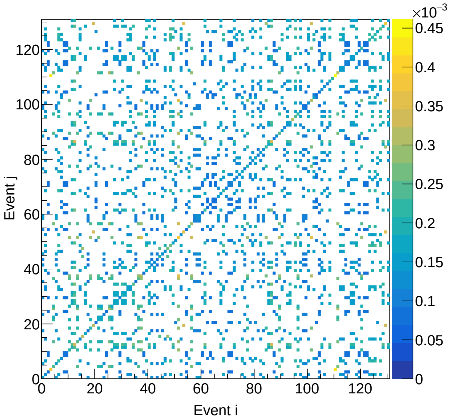
LD2 (total) Covariance | M: [5.7, 6.0) xF: [0.45, 0.50)
