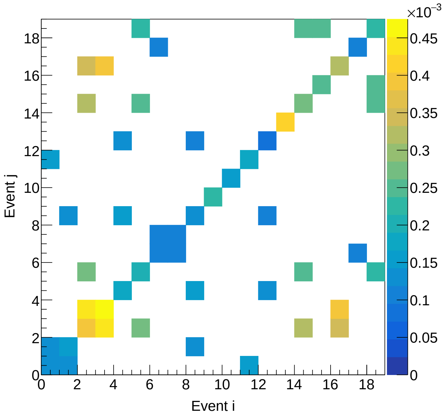
LD2 (total) Covariance | M: [6.9, 7.5) xF: [0.50, 0.55)
