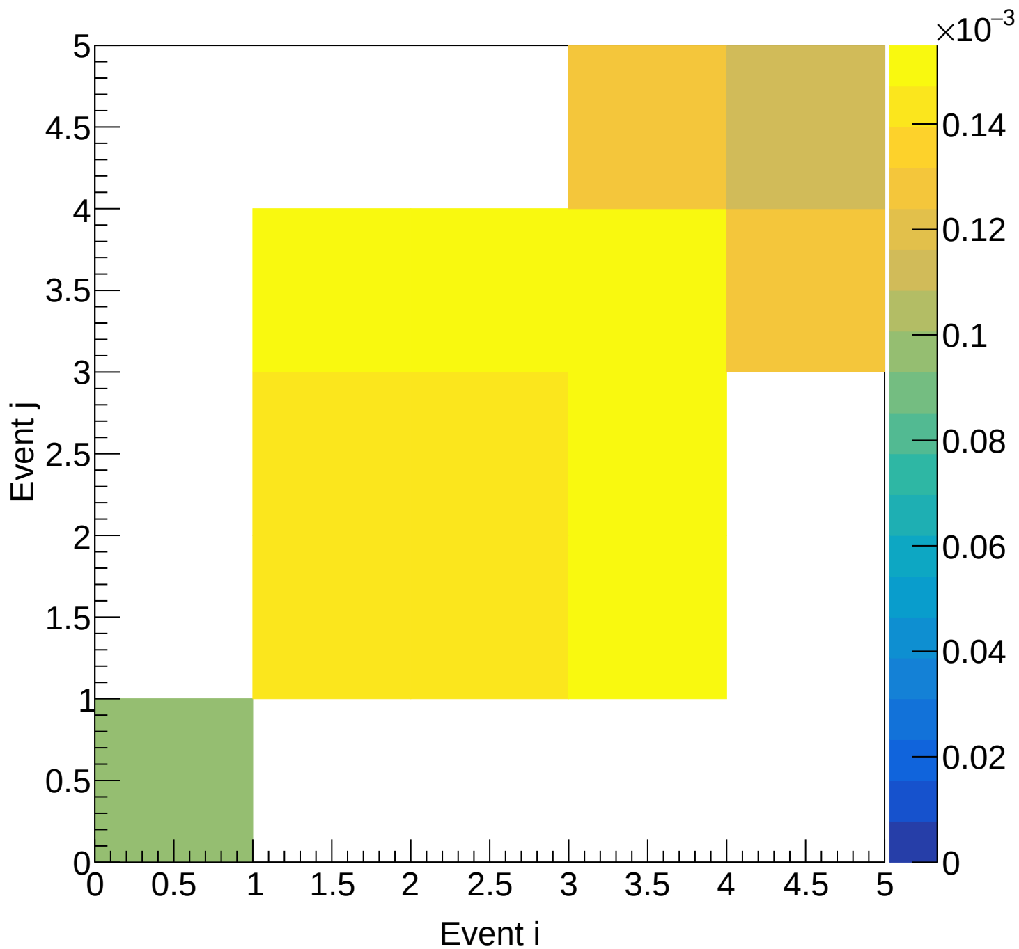
LD2 (total) Covariance | M: [7.5, 8.8) xF: [0.50, 0.55)
