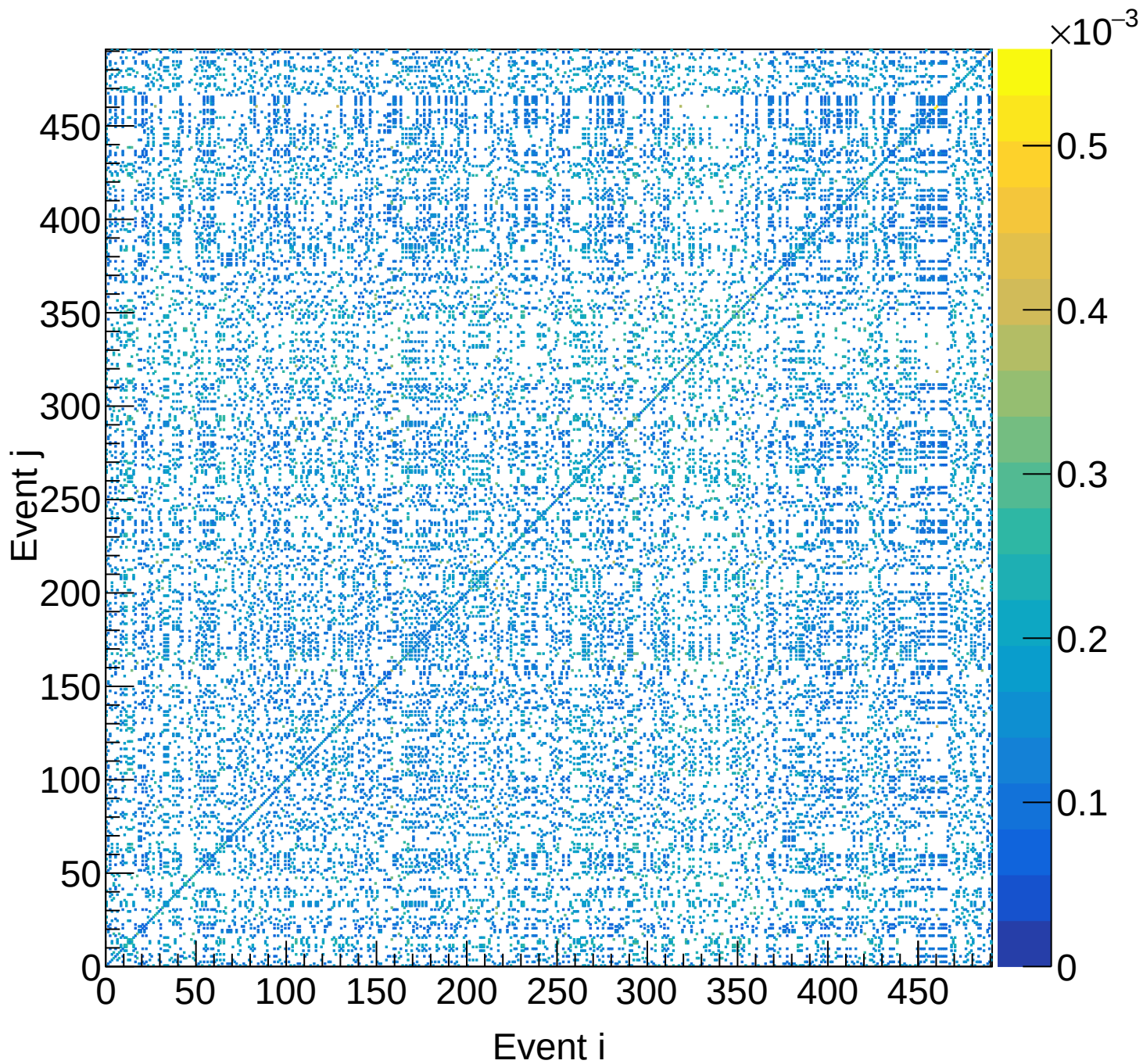
LD2 (total) Covariance | M: [4.5, 4.8) xF: [0.50, 0.55)
