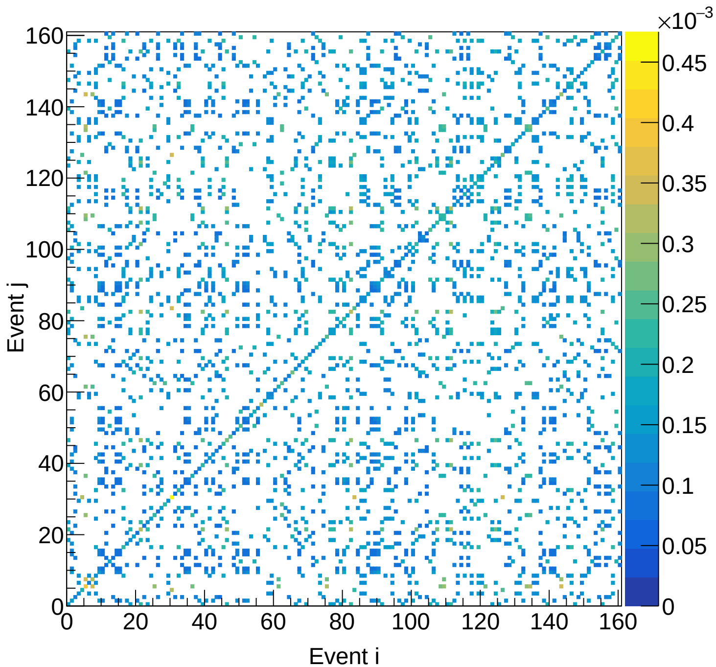
LD2 (total) Covariance | M: [5.4, 5.7) xF: [0.50, 0.55)
