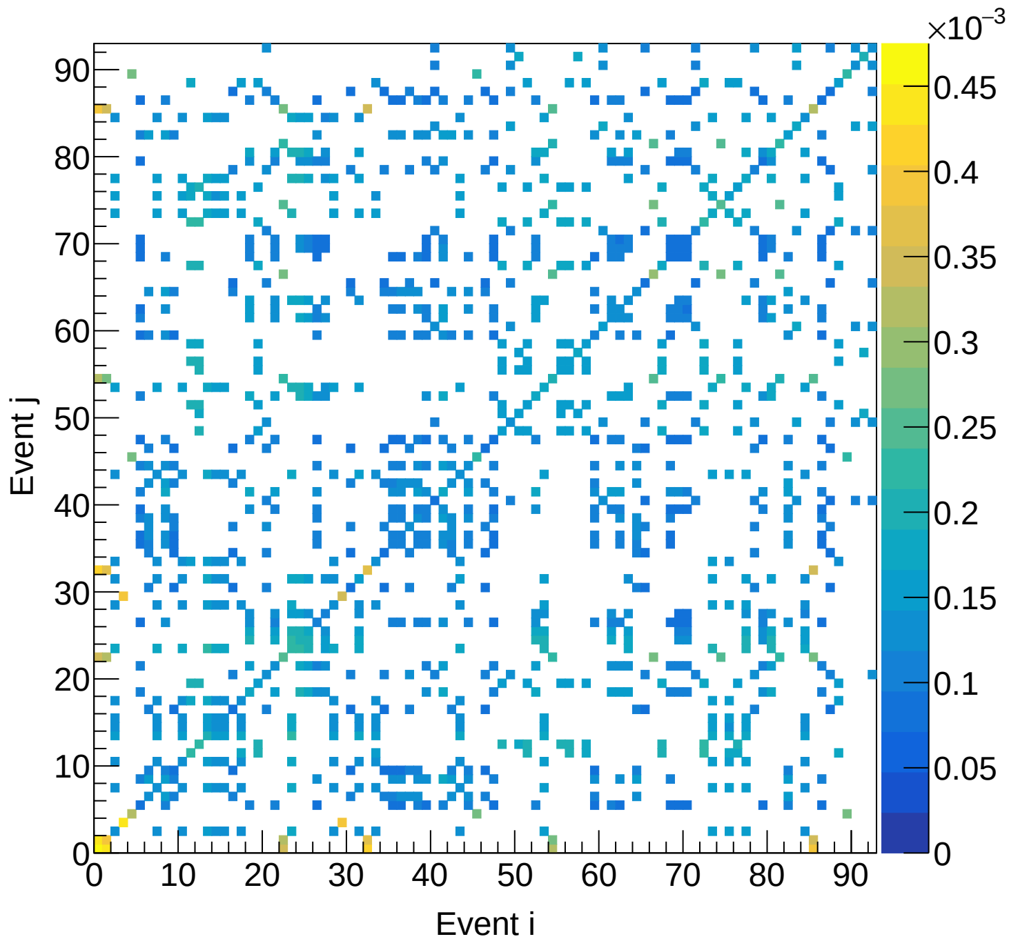
LD2 (total) Covariance | M: [5.7, 6.0] xF: [0.50, 0.55]
