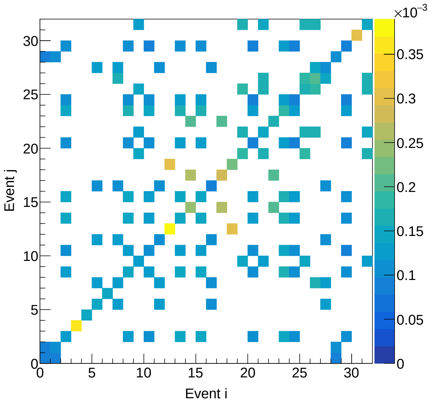
LD2 (total) Covariance | M: [6.6, 6.9] xF: [0.50, 0.55]
