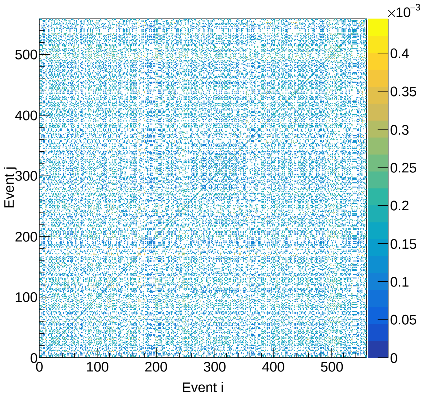
LD2 (total) Covariance | M: [4.2, 4.5) xF: [0.55, 0.60)
