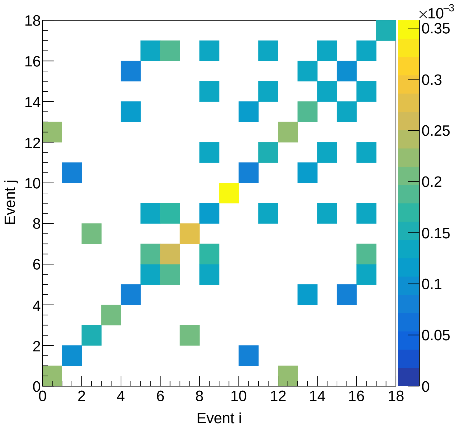
LD2 (total) Covariance | M: [6.9, 7.5) xF: [0.55, 0.60)
