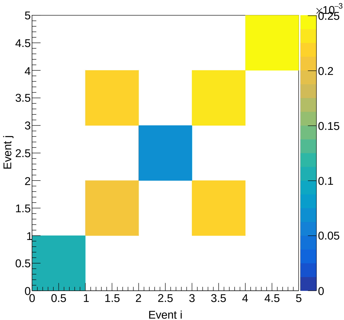
LD2 (total) Covariance | M: [7.5, 8.8) xF: [0.55, 0.60)
