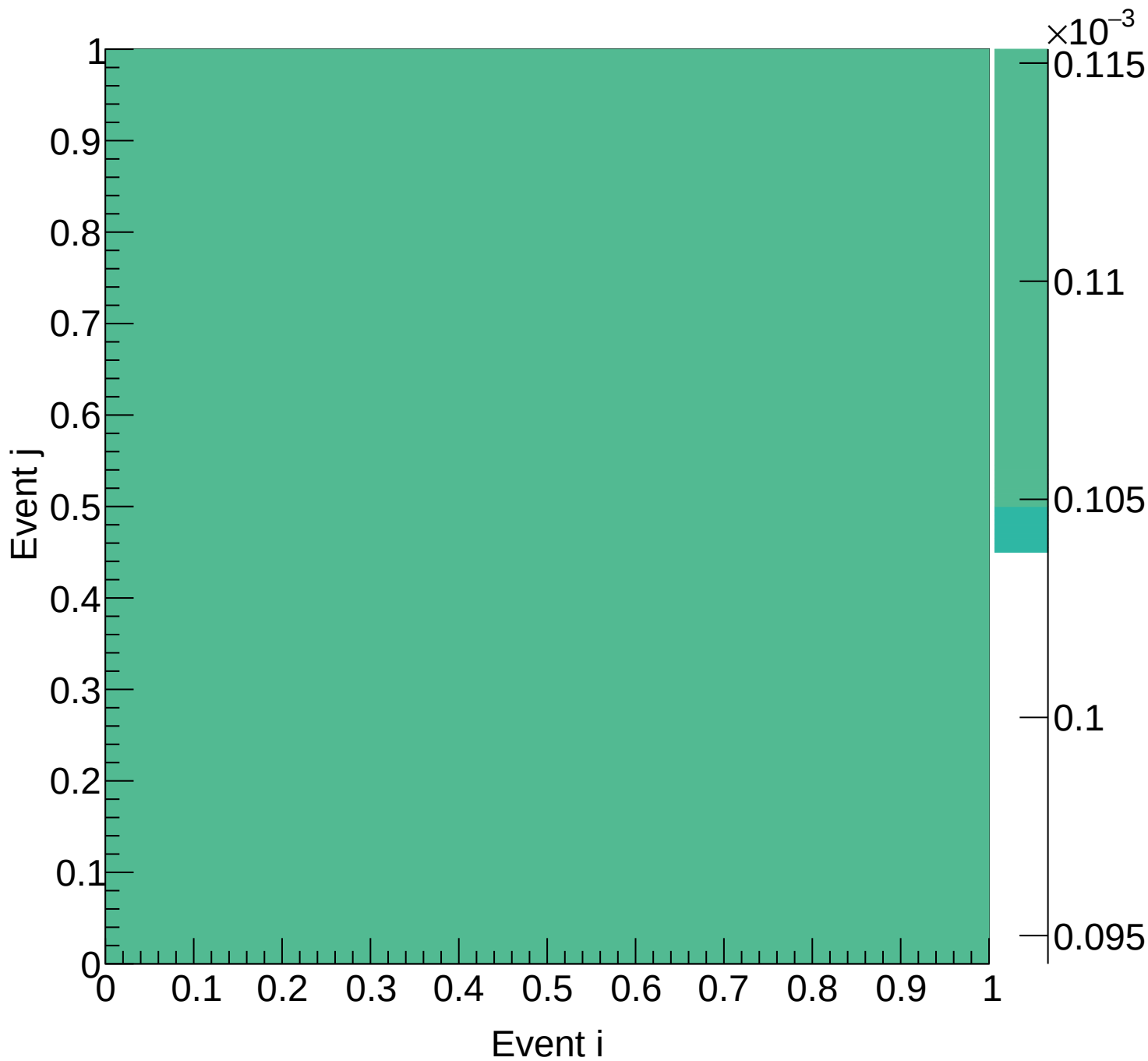
LD2 (total) Covariance | M: [8.8, 10.0) xF: [0.55, 0.60)
