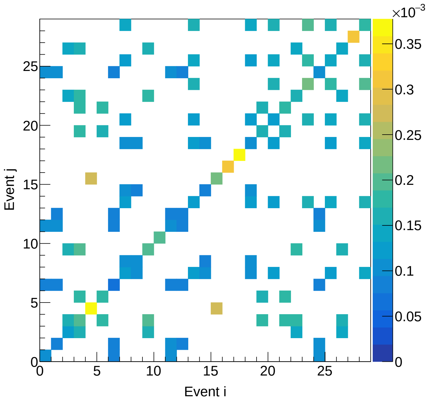
LD2 (total) Covariance | M: [6.3, 6.6] xF: [0.55, 0.60]
