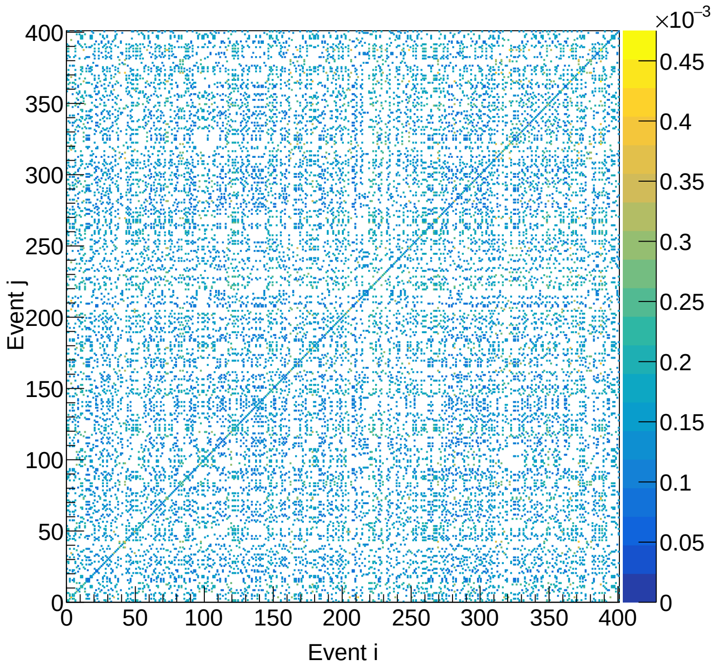
LD2 (total) Covariance | M: [4.2, 4.5) xF: [0.60, 0.65)
