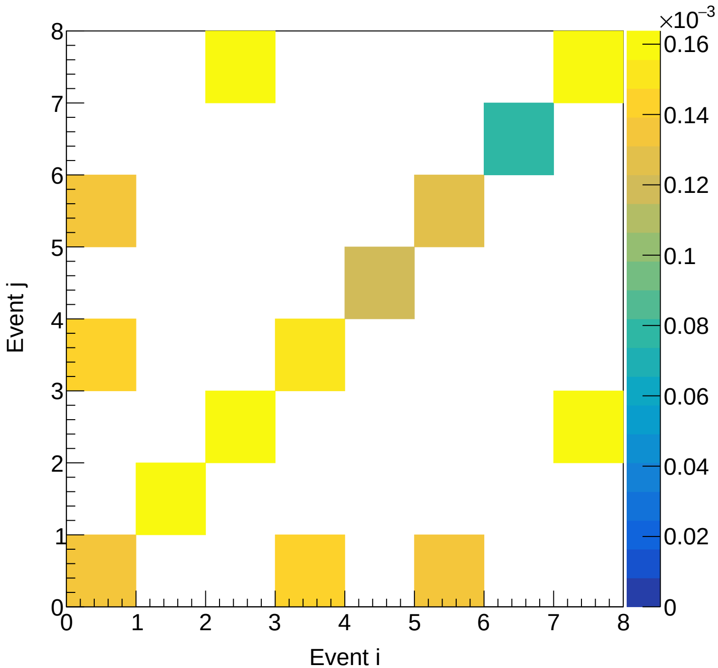
LD2 (total) Covariance | M: [6.9, 7.5) xF: [0.60, 0.65)
