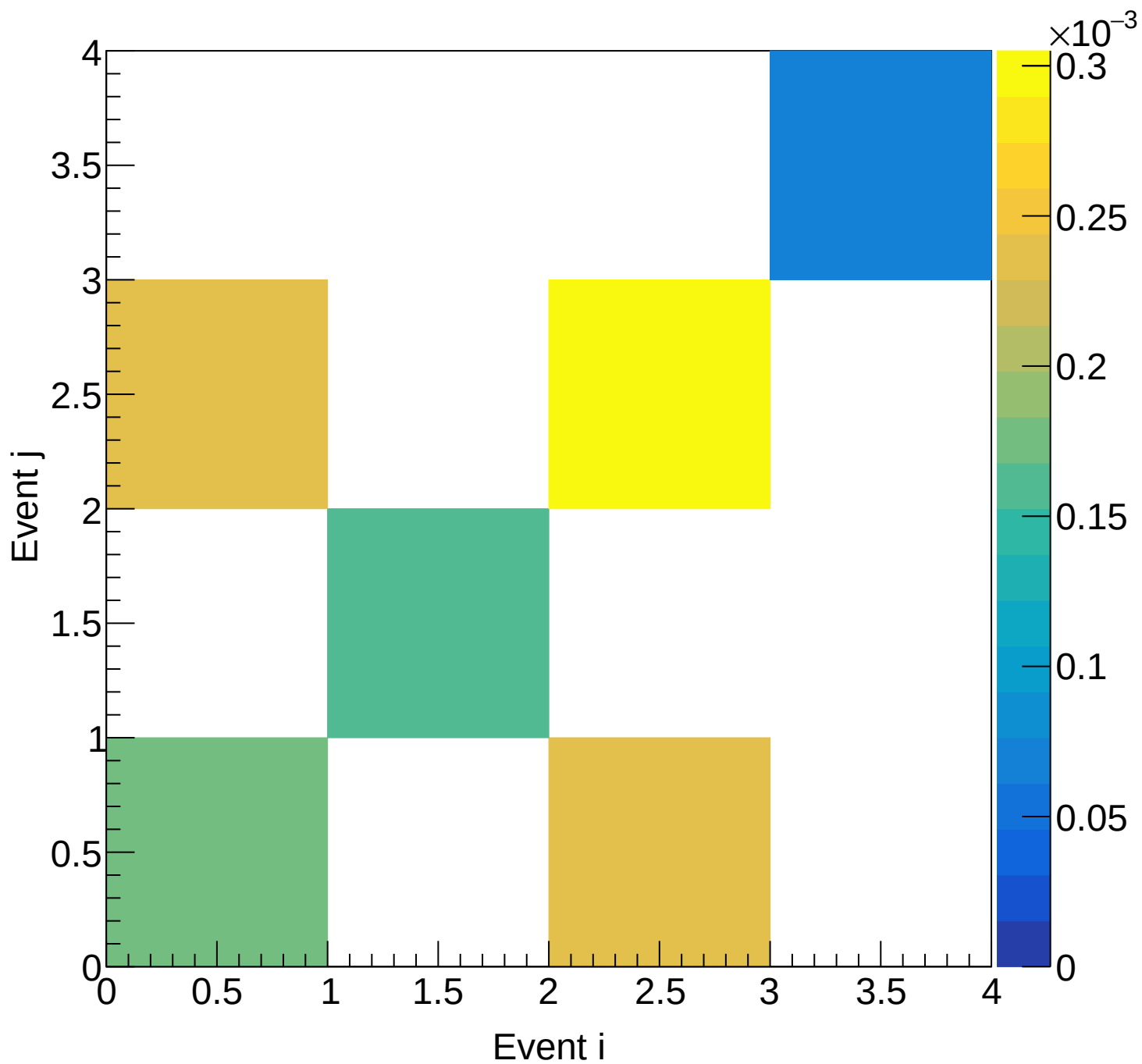
LD2 (total) Covariance | M: [7.5, 8.8) xF: [0.60, 0.65)
