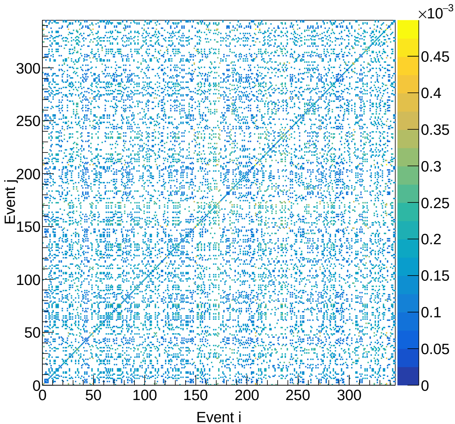
LD2 (total) Covariance | M: [4.5, 4.8) xF: [0.60, 0.65)
