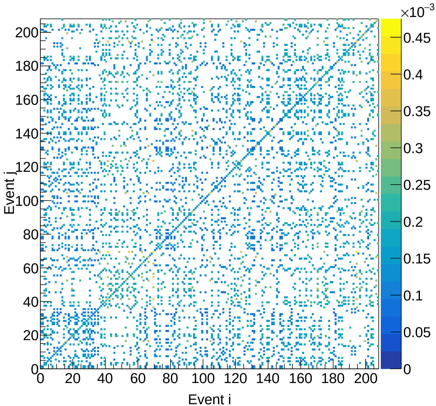
LD2 (total) Covariance | M: [4.8, 5.1) xF: [0.60, 0.65)
