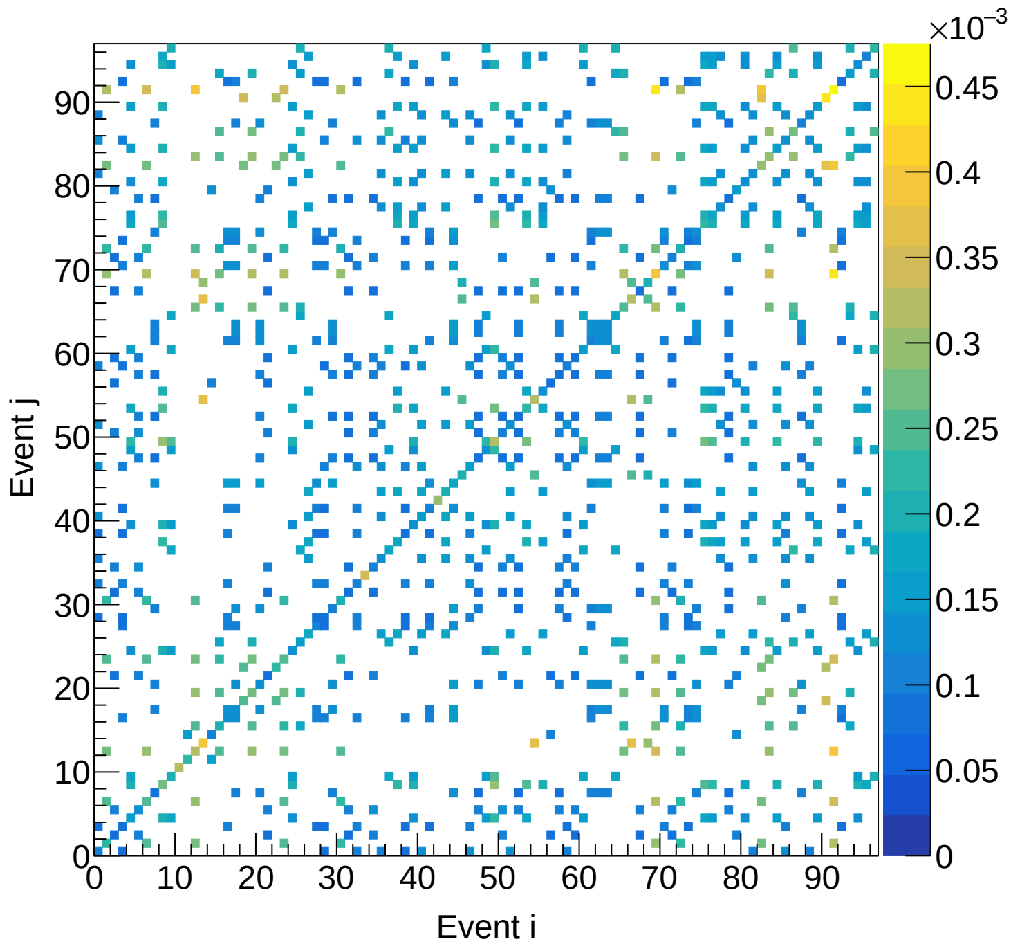
LD2 (total) Covariance | M: [5.4, 5.7) xF: [0.60, 0.65)
