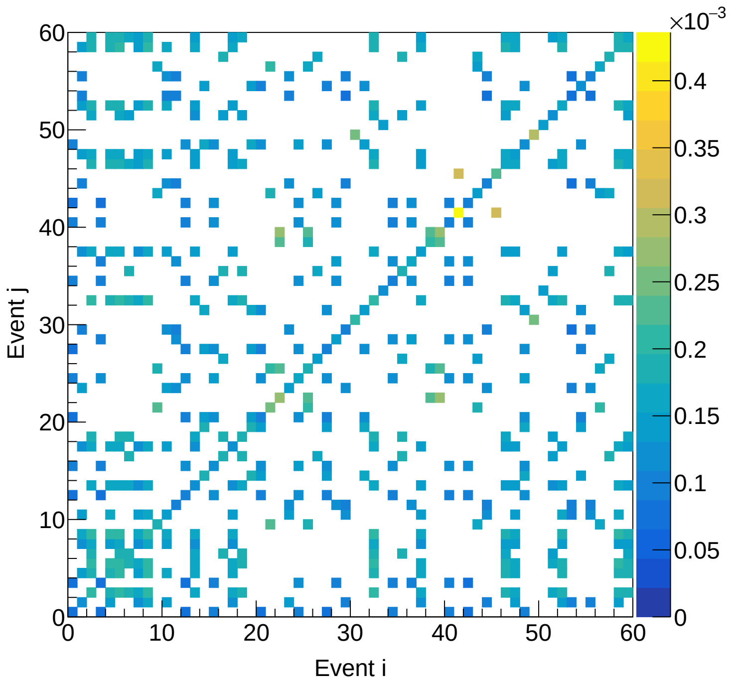
LD2 (total) Covariance | M: [5.7, 6.0) xF: [0.60, 0.65)
