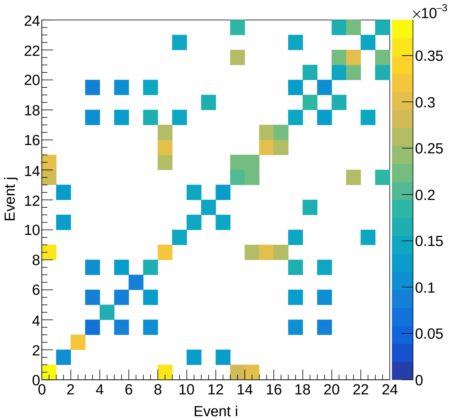
LD2 (total) Covariance | M: [6.3, 6.6) xF: [0.60, 0.65)
