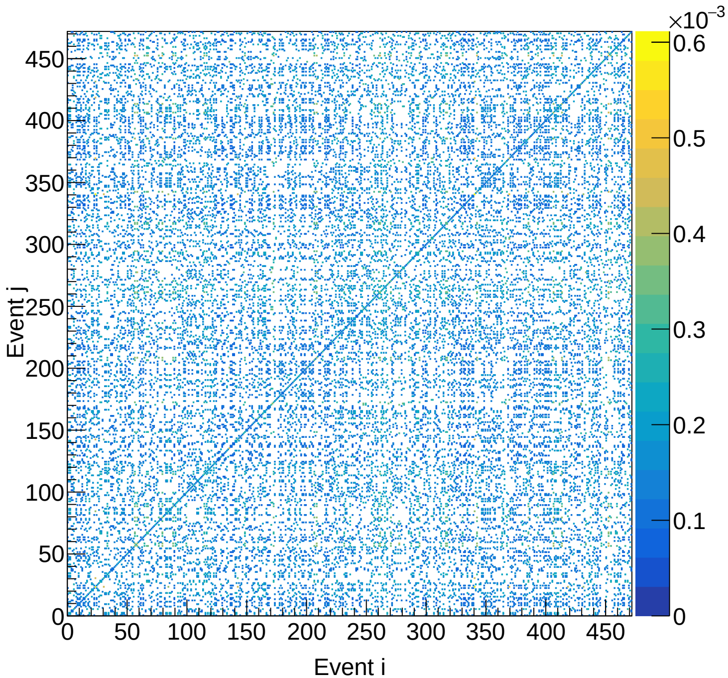
LD2 (total) Covariance | M: [3.9, 4.2) xF: [0.65, 0.70)
