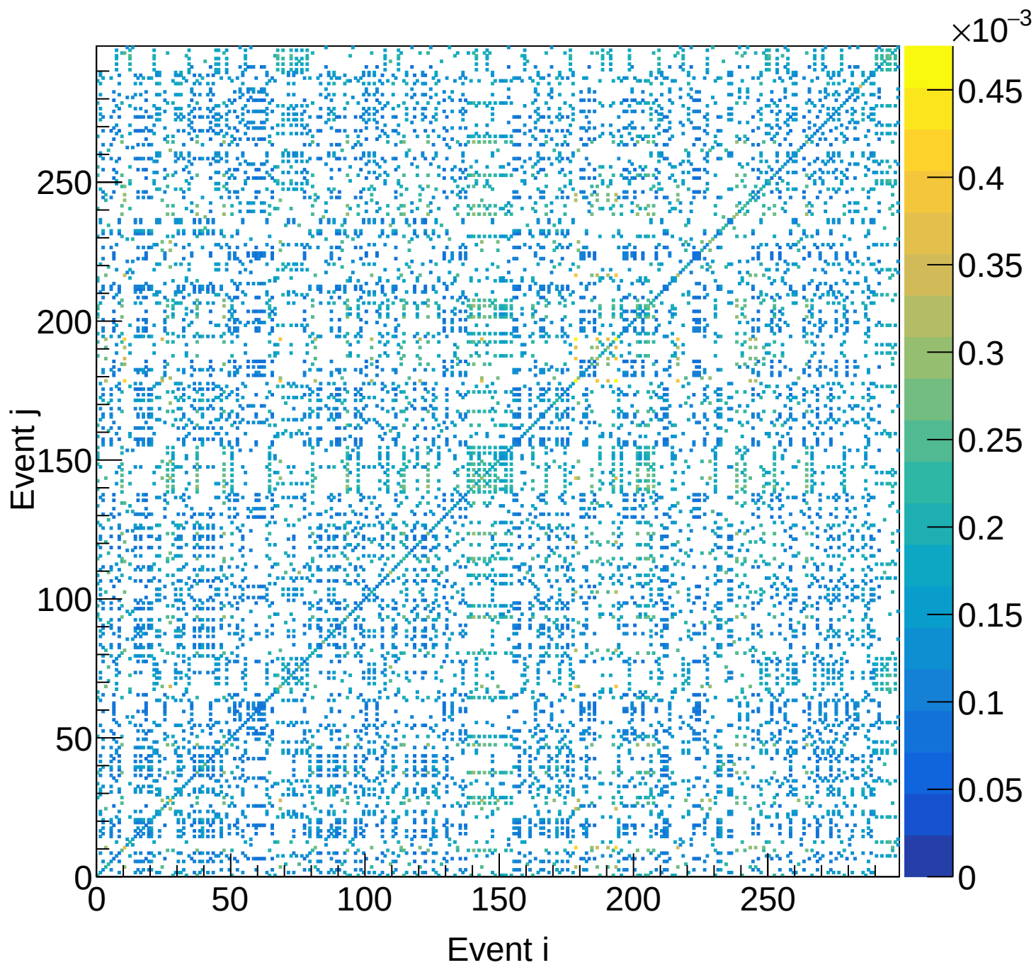
LD2 (total) Covariance | M: [4.2, 4.5] xF: [0.65, 0.70)
