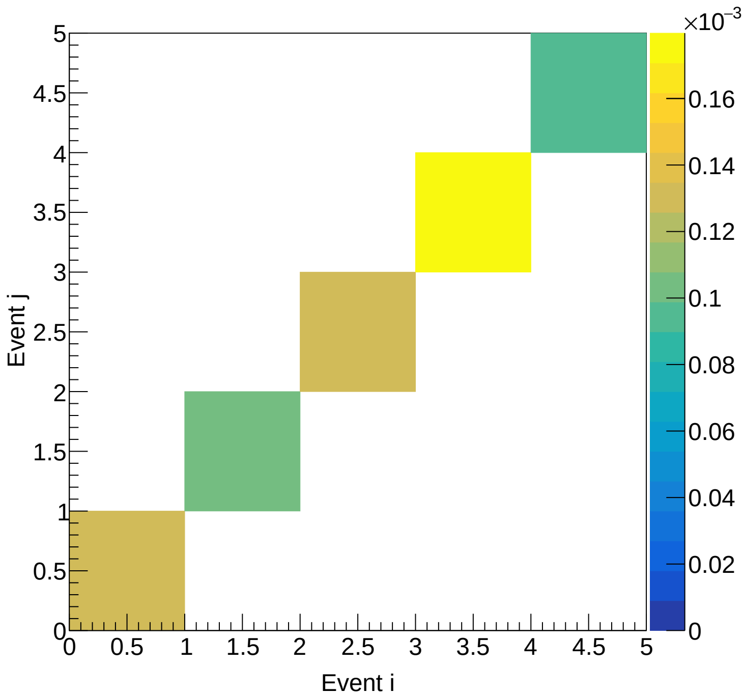
LD2 (total) Covariance | M: [6.9, 7.5) xF: [0.65, 0.70)
