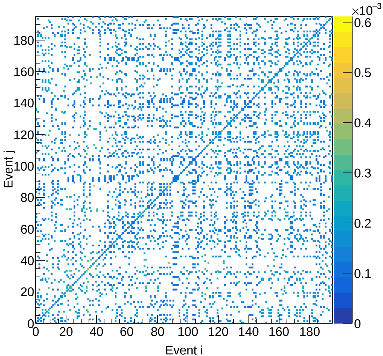
LD2 (total) Covariance | M: [4.5, 4.8) xF: [0.65, 0.70)
