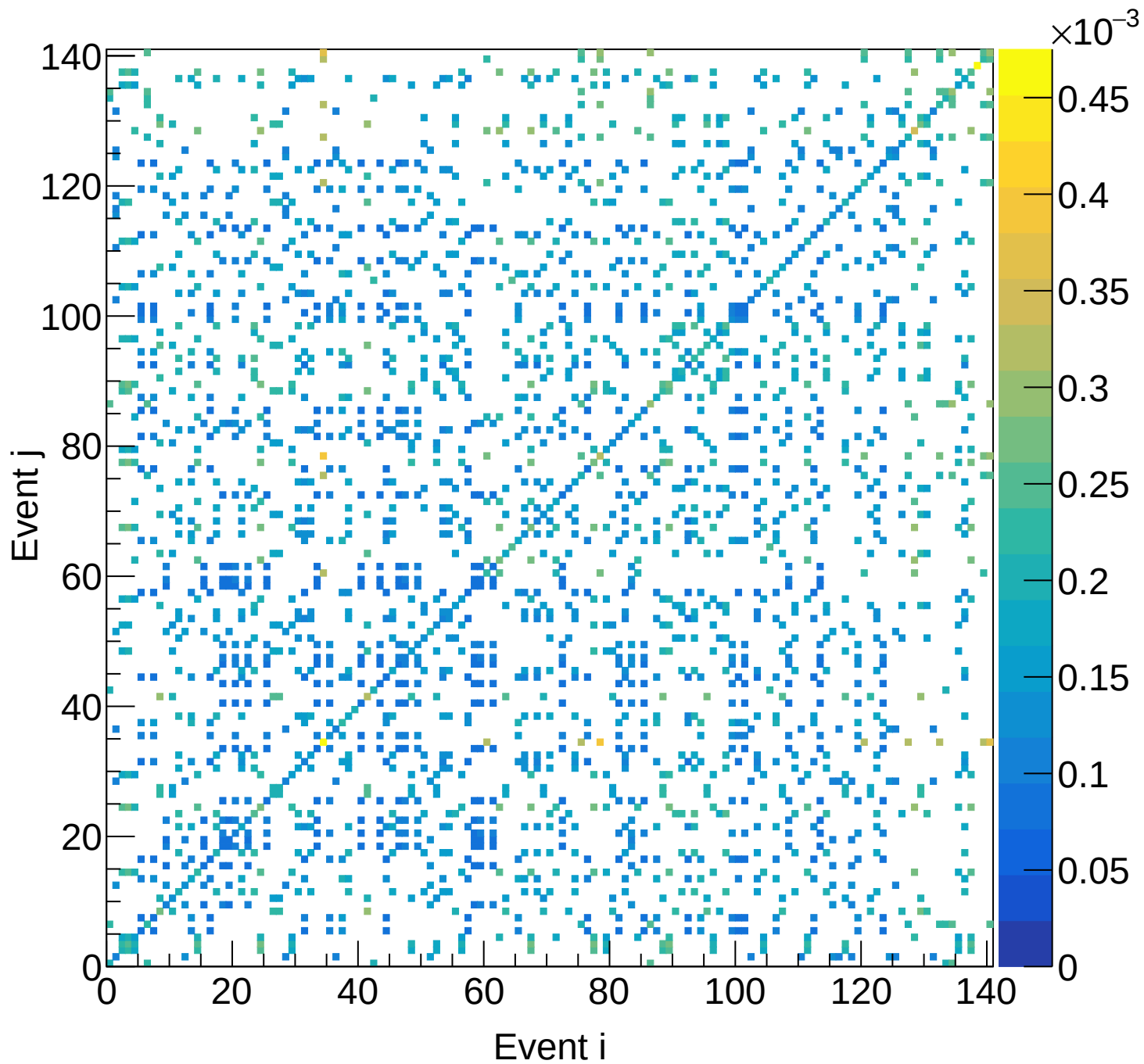
LD2 (total) Covariance | M: [4.8, 5.1) xF: [0.65, 0.70)
