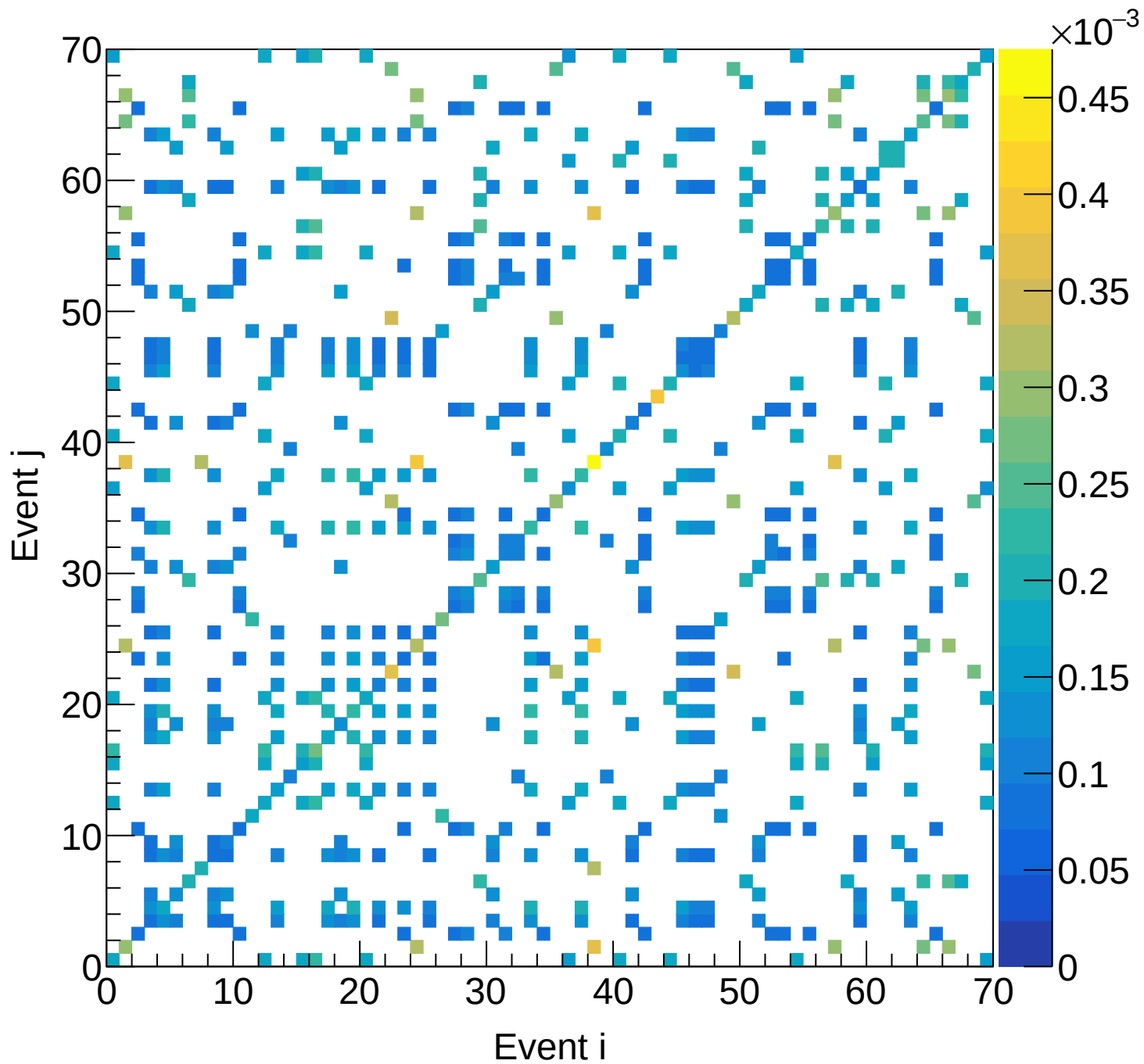
LD2 (total) Covariance | M: [5.1, 5.4) xF: [0.65, 0.70)
