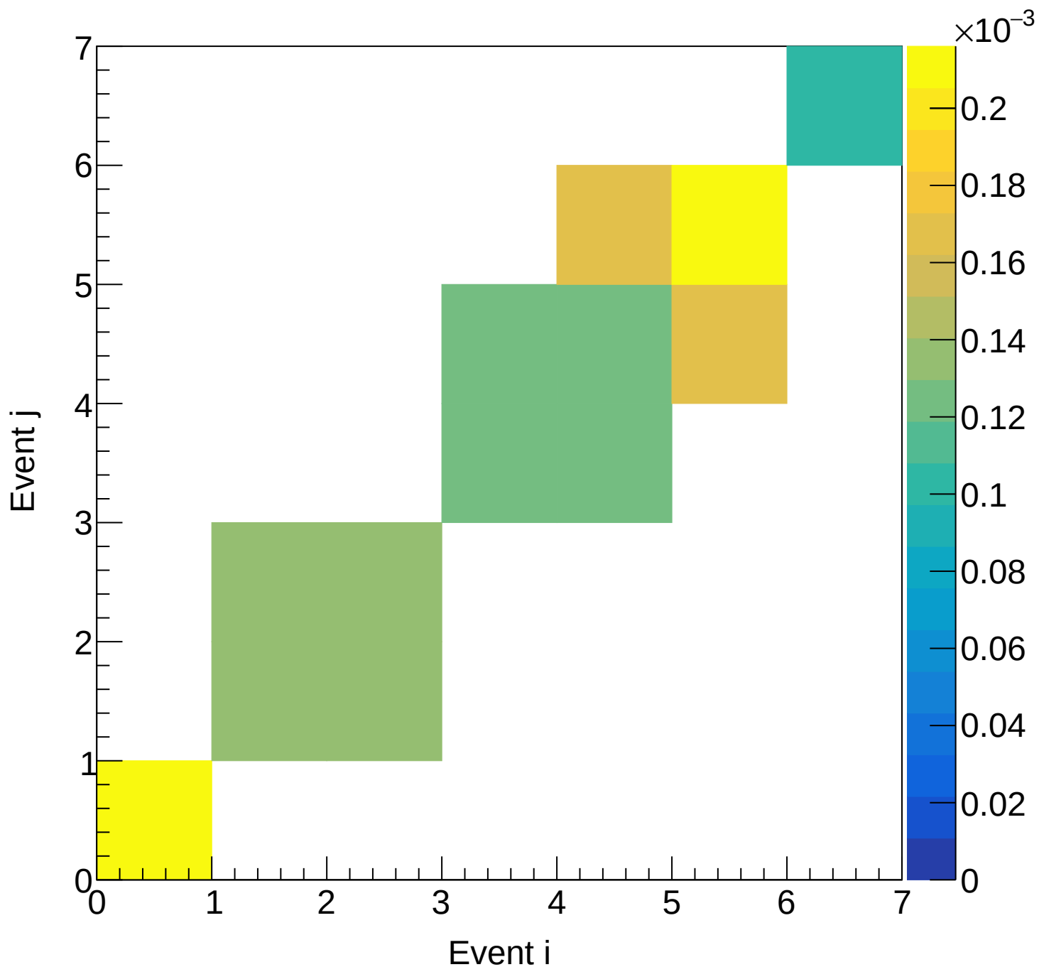
LD2 (total) Covariance | M: [6.3, 6.6) xF: [0.65, 0.70)
