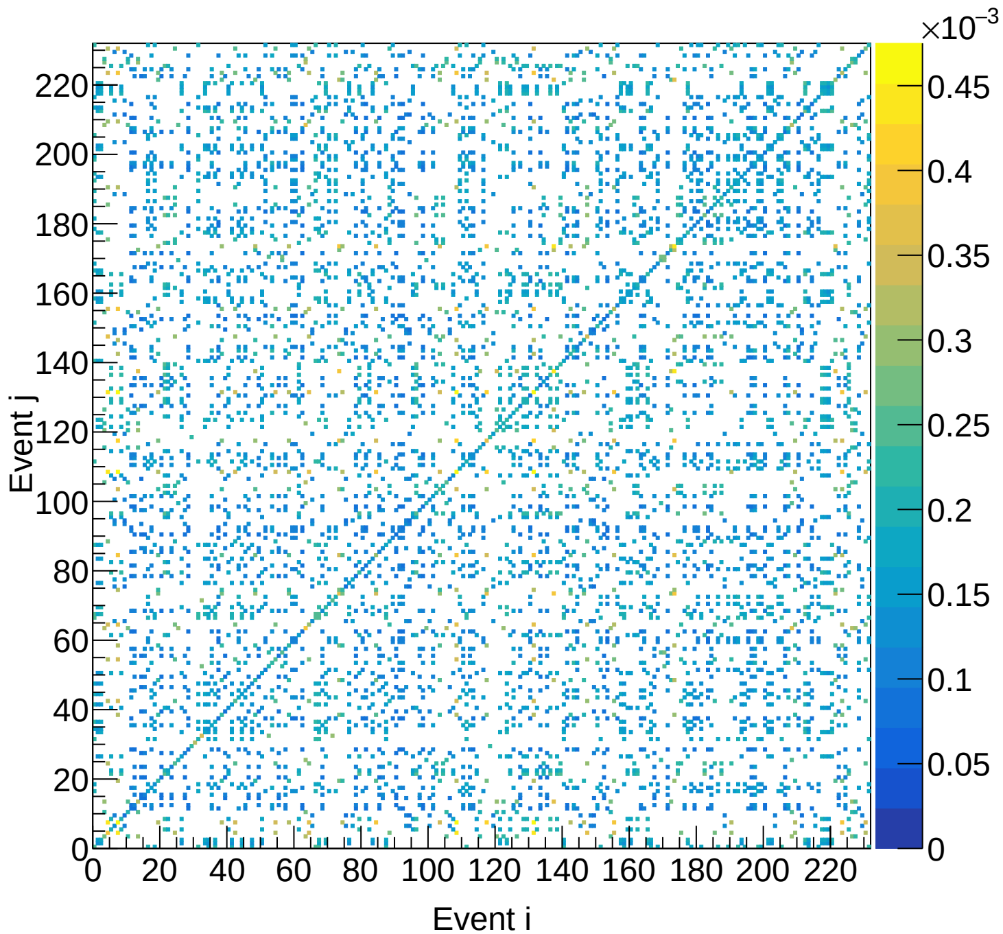
LD2 (total) Covariance | M: [3.9, 4.2) xF: [0.70, 0.75)
