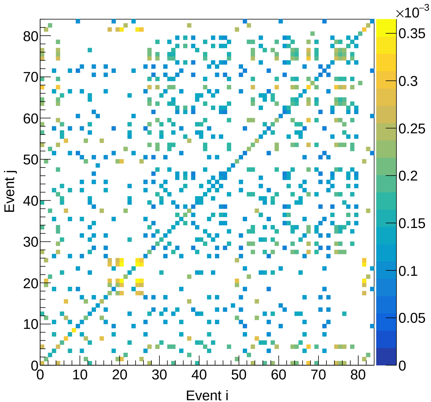
LD2 (total) Covariance | M: [4.8, 5.1) xF: [0.70, 0.75)
