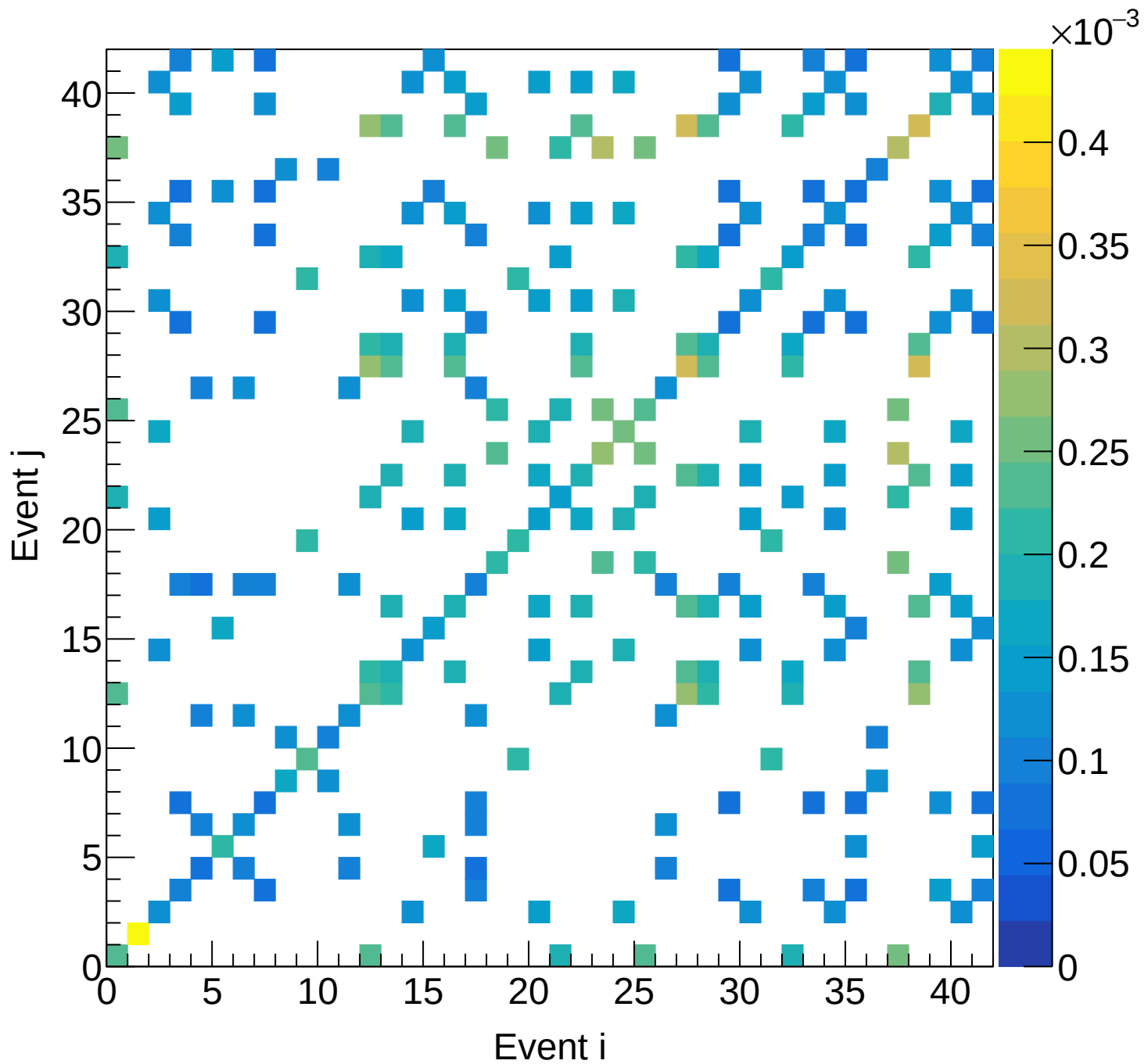
LD2 (total) Covariance | M: [5.4, 5.7] xF: [0.70, 0.75]
