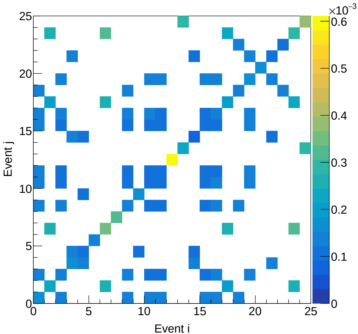
LD2 (total) Covariance | M: [5.7, 6.0] xF: [0.70, 0.75)
