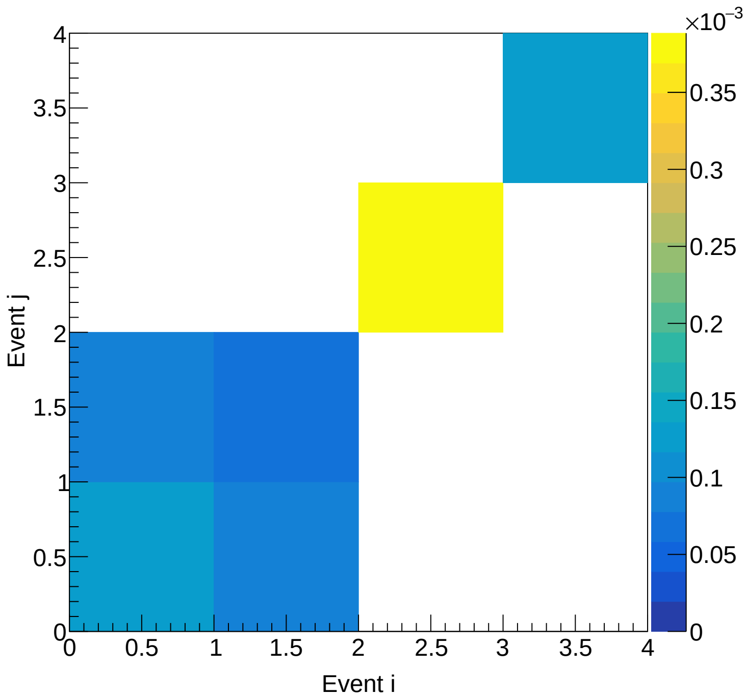
LD2 (total) Covariance | M: [6.6, 6.9] xF: [0.70, 0.75]
