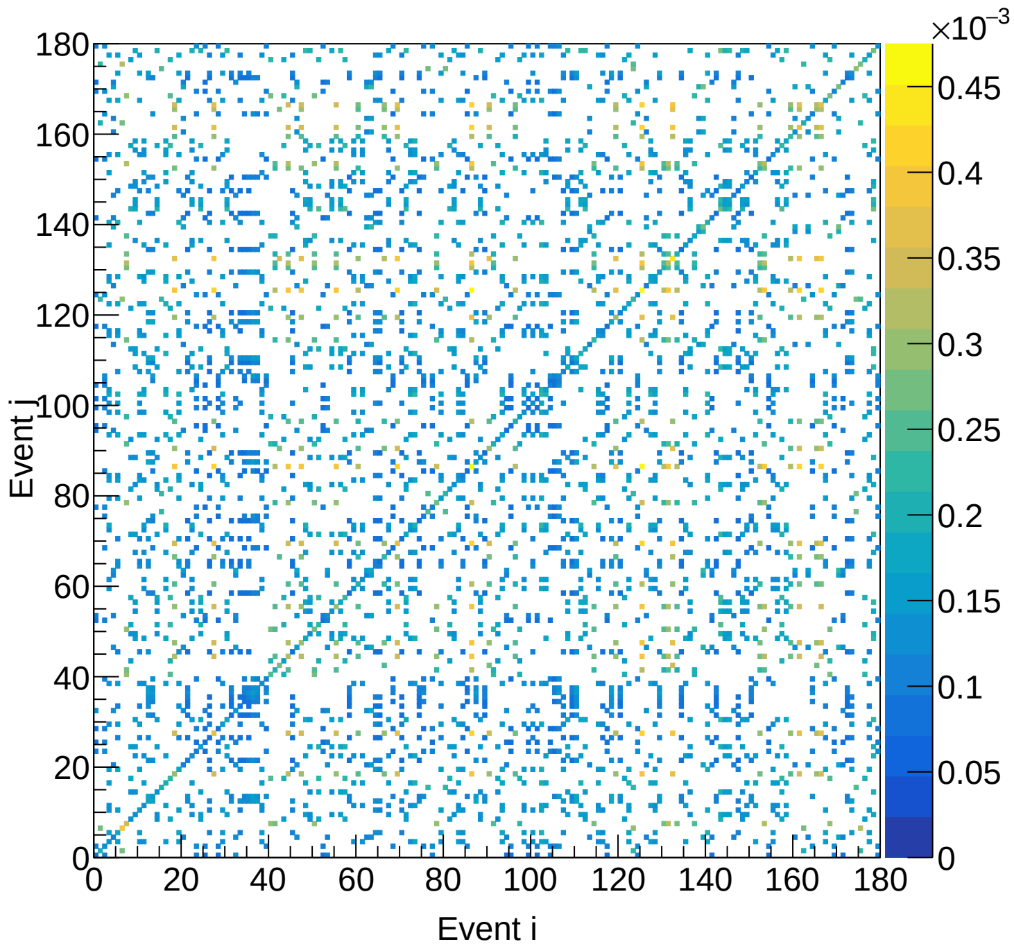
LD2 (total) Covariance | M: [3.9, 4.2) xF: [0.75, 0.80)
