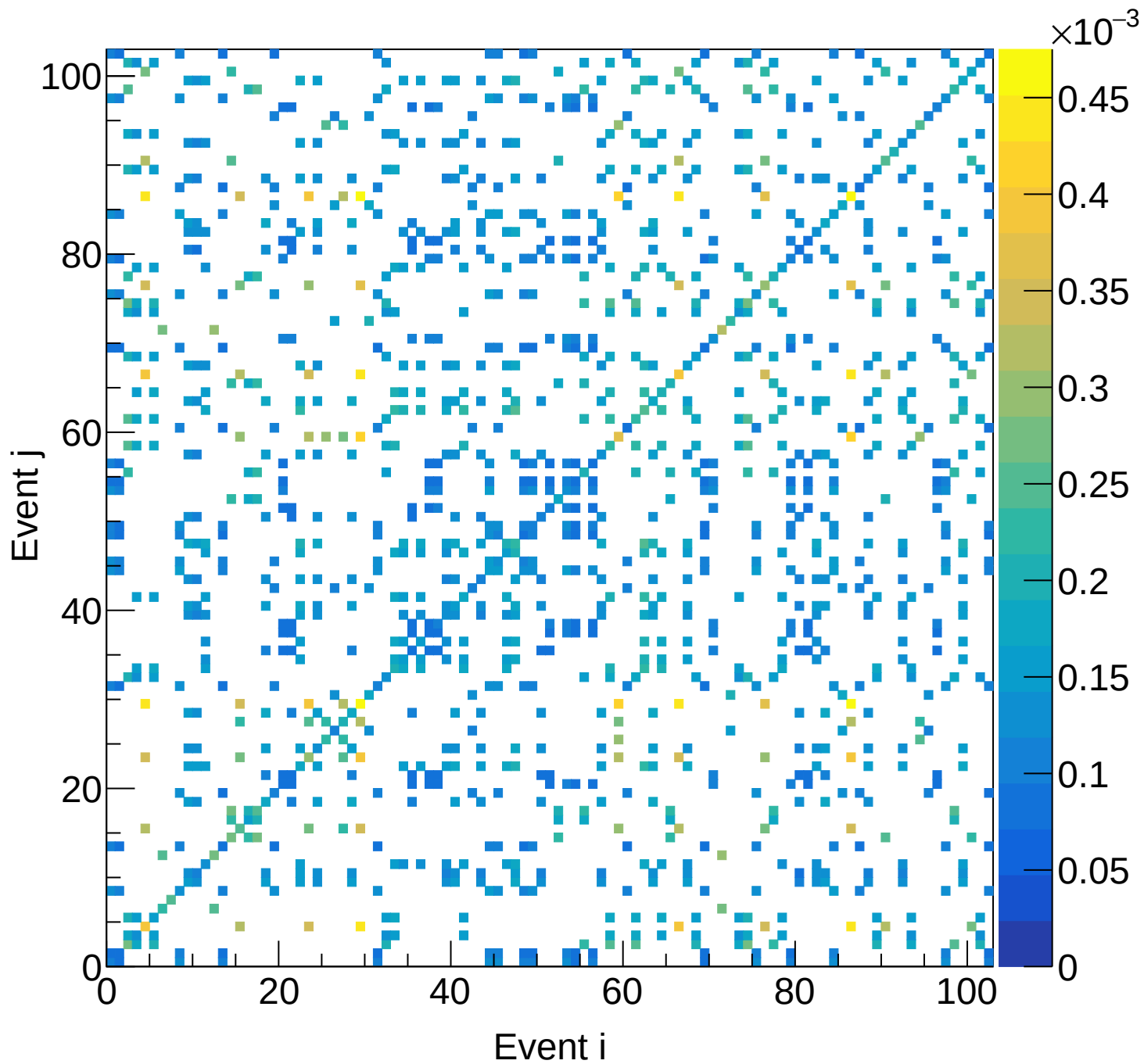
LD2 (total) Covariance | M: [4.2, 4.5) xF: [0.75, 0.80)
