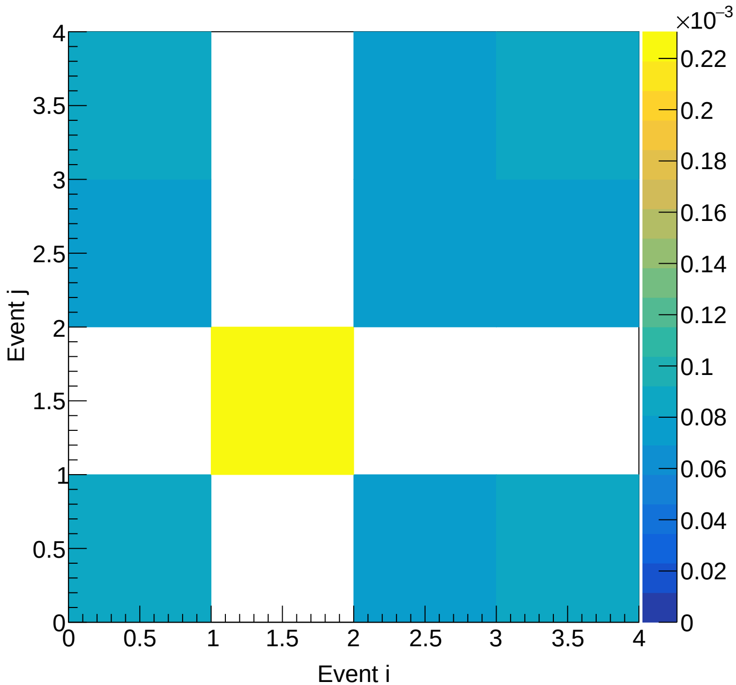
LD2 (total) Covariance | M: [7.5, 8.8) xF: [0.75, 0.80)
