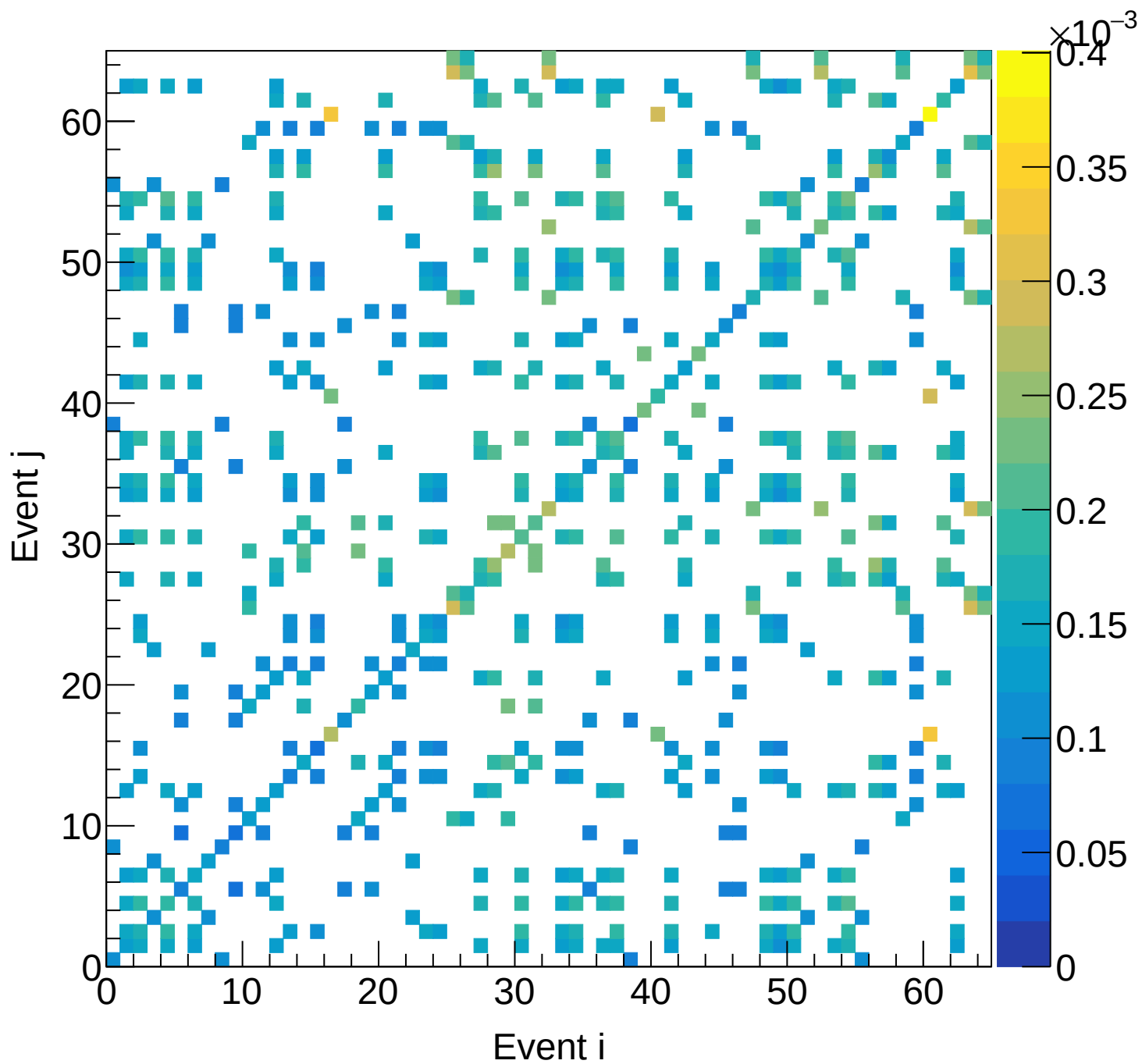
LD2 (total) Covariance | M: [4.5, 4.8) xF: [0.75, 0.80)
