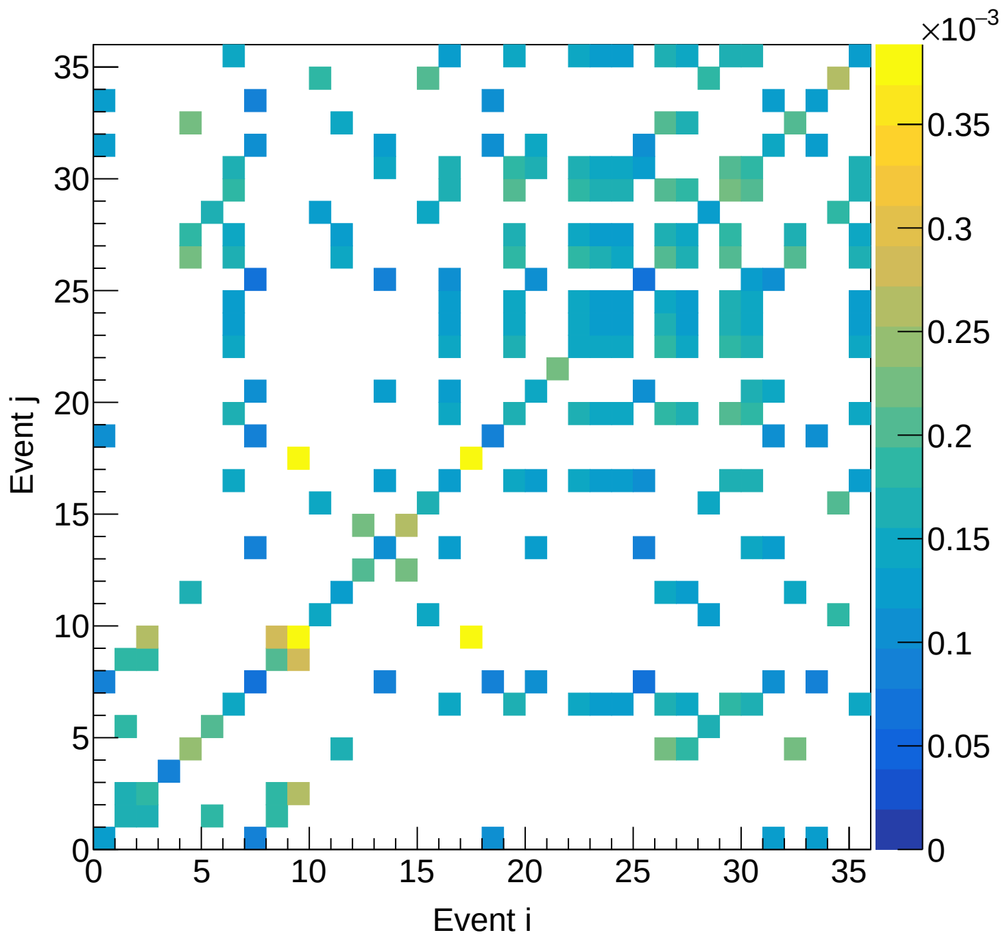
LD2 (total) Covariance | M: [5.1, 5.4) xF: [0.75, 0.80)
