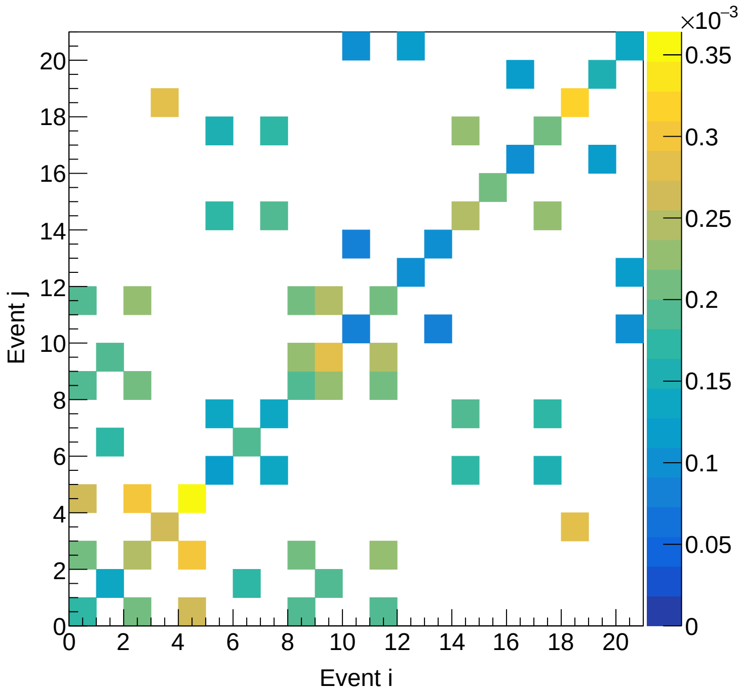
LD2 (total) Covariance | M: [5.4, 5.7) xF: [0.75, 0.80)
