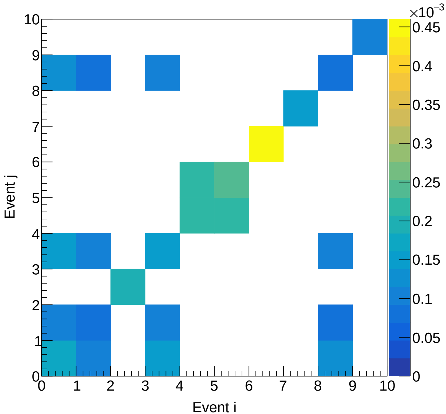
LD2 (total) Covariance | M: [6.0, 6.3) xF: [0.75, 0.80)
