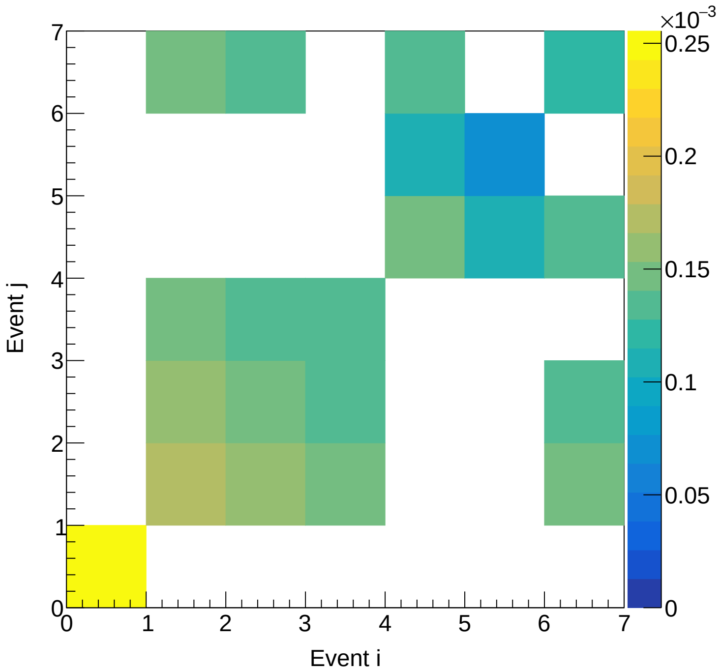
LD2 (total) Covariance | M: [6.3, 6.6) xF: [0.75, 0.80)
