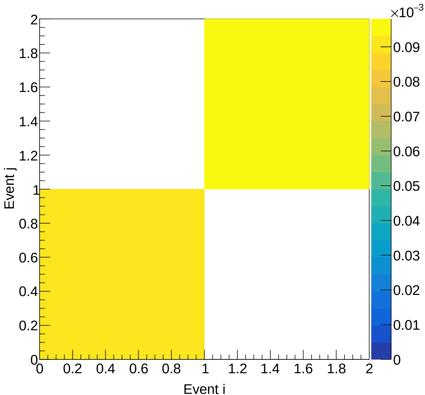
LD2 (total) Covariance | M: [6.6, 6.9] xF: [0.75, 0.80)
