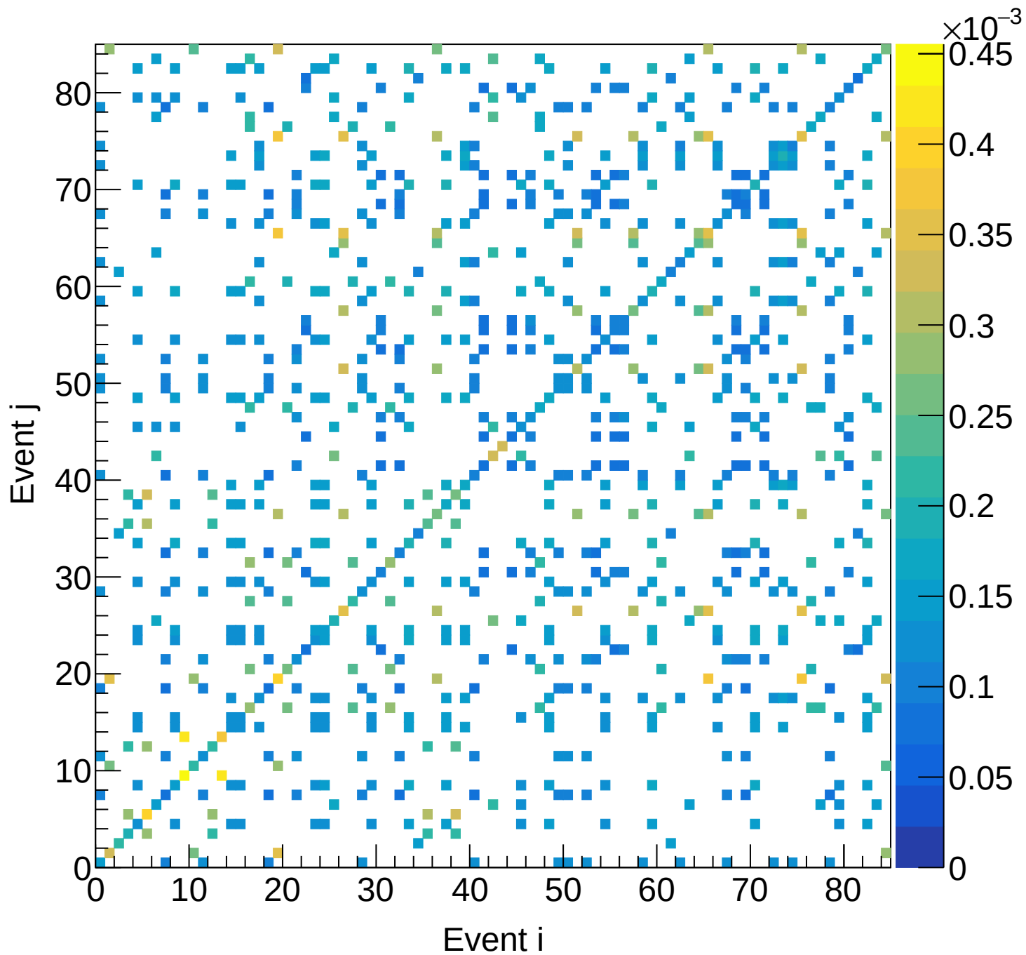
LD2 (total) Covariance | M: [3.9, 4.2] xF: [0.80, 0.85]
