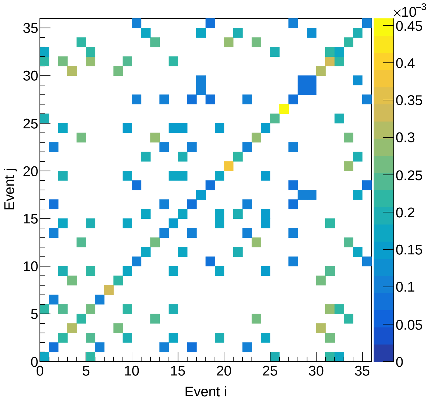
LD2 (total) Covariance | M: [4.2, 4.5) xF: [0.80, 0.85)
