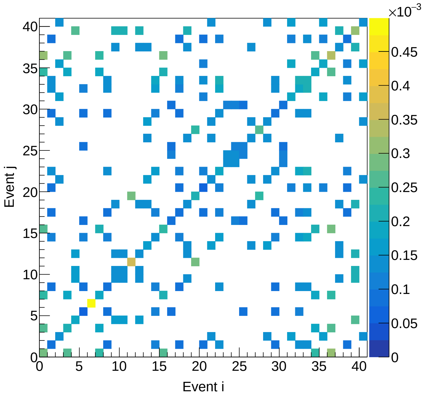
LD2 (total) Covariance | M: [4.5, 4.8) xF: [0.80, 0.85)
