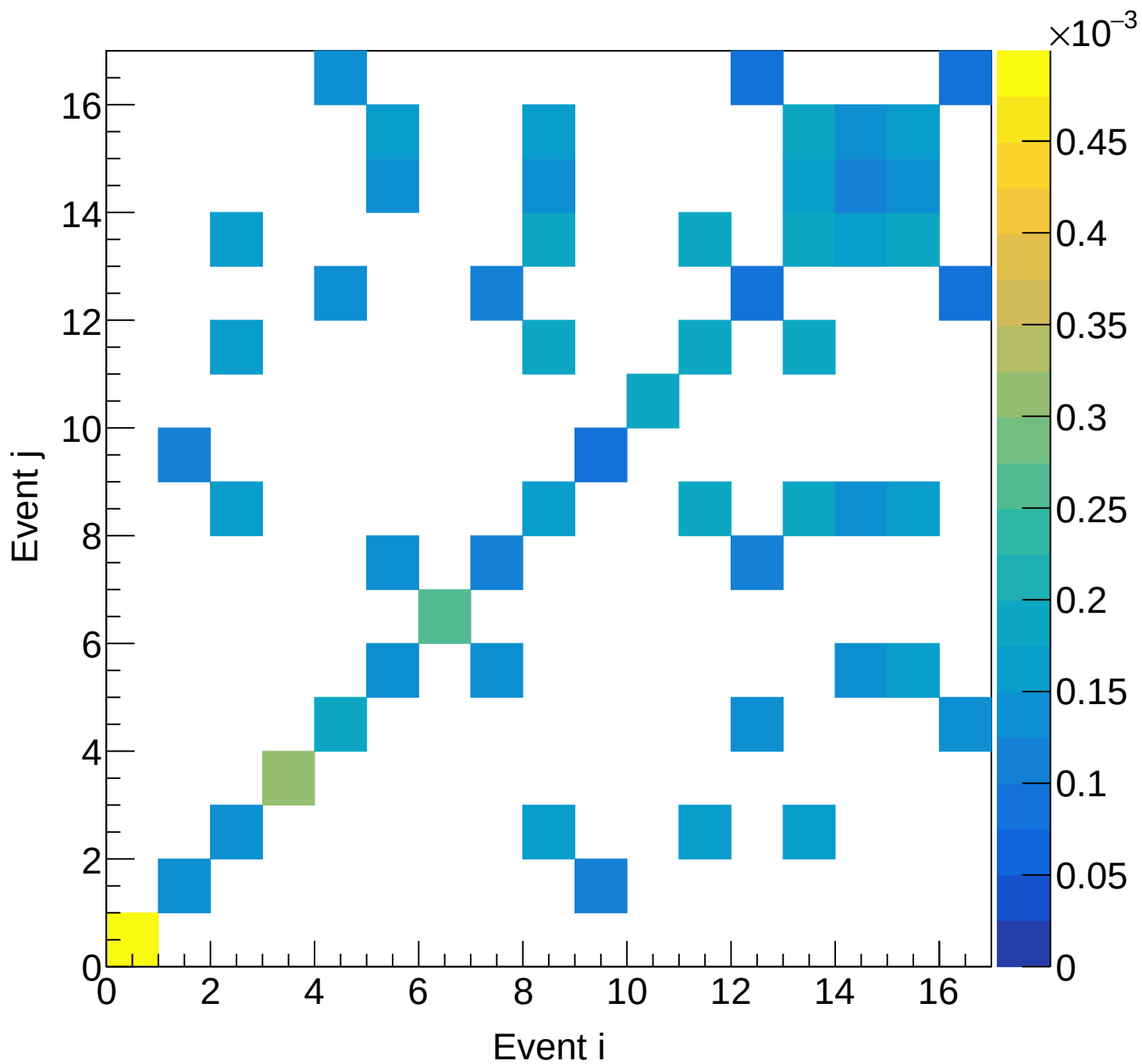
LD2 (total) Covariance | M: [4.8, 5.1) xF: [0.80, 0.85)
